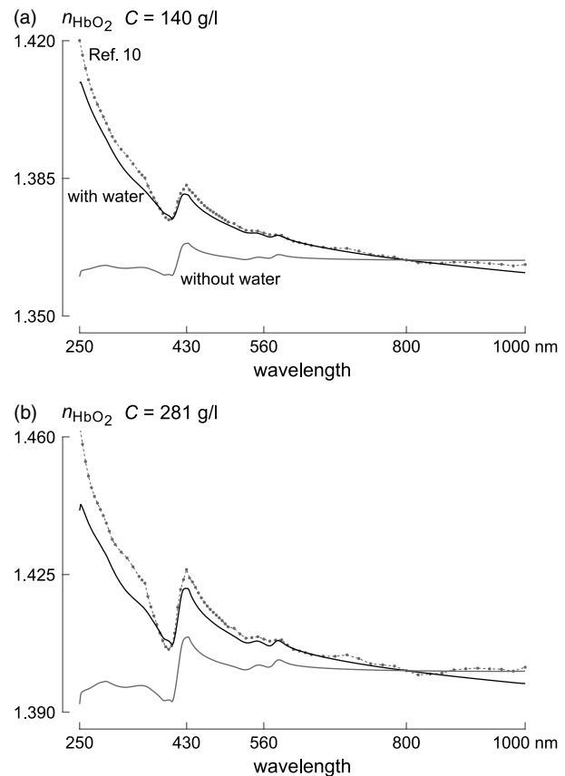
Fig. 3 The real part of the refractive index obtained by the Kramers-Kronig analysis with the water contribution taken into account (black lines) agrees with the results of the model functions of Friebel and Meinke (gray dots). 10 They disagree when the water contribution is ignored (gray lines). The hemoglobin concentration is 140 g/l in (a) and 281 g/l in (b).
