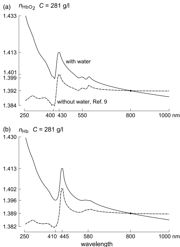
Fig. 2 The refractive index for (a) oxygenated and (b) deoxygenated hemoglobin solutions obtained from the Kramers-Kronig relations. The calculations took the water contribution into account for the solid black lines and ignored it for the gray lines. The gray lines almost coincide with the dashed black lines that are taken from Ref. 9. The hemoglobin concentration is 281 g/l.
