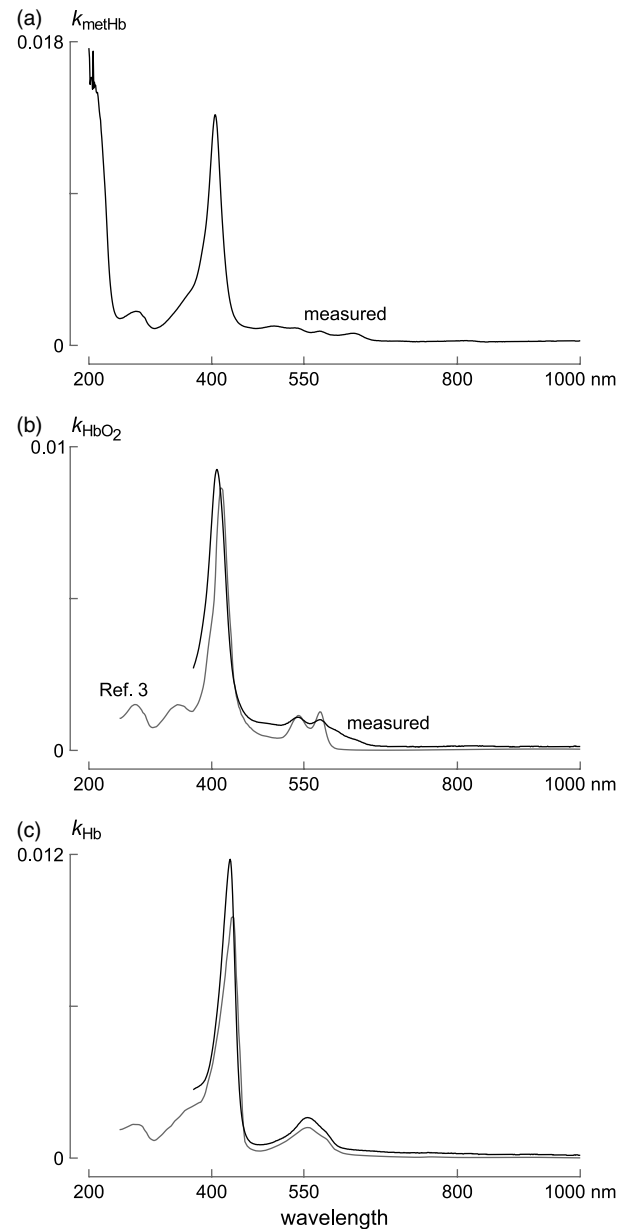
Fig. 1 Measured values (black lines) of the imaginary part of the refractive index of (a) methemoglobin; (b) oxygenated; and (c) deoxygenated hemoglobin solutions. The hemoglobin concentration is 140 g/l. Gray lines are calculated from the tabulated data of Ref. 3.
