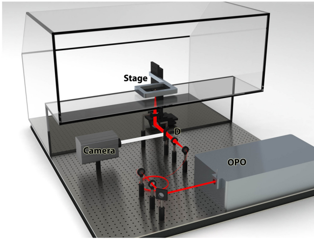
Fig. 1 Experimental setup used to measure the thermal response of tissue to laser exposure. OPO, optical parametric oscillator; D, dichroic; and Camera, FLIR thermal camera. The red beam corresponds to the excitation path and the white beam corresponds to the collected thermal signal (3 to 5 \mu\text{m} ).
