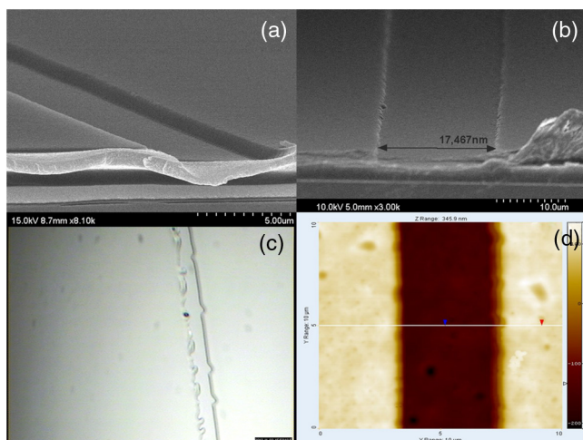
Fig. 3 The NIL-patterned waveguide channel in the DNA biopolymer with (a) “excellent” imprint quality (SEM image), (b) “good” imprint quality (SEM image), (c) “poor” imprint quality of 15- \mu\text{m} wide channel (micrograph), and (d) “good” imprint quality (AFM image). The imprint quality descriptors “excellent,” “good,” and “poor” are defined in the text.
