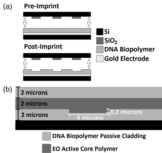
Fig. 1 (a) Schematic of the nanoimprint lithography (NIL) process showing the deoxyribonucleic acid (DNA) biopolymer film pre- and postimprint (b) the electro-optic (EO) modulator waveguide device structure with a DNA biopolymer cladding on either side of the EO active core polymer.
