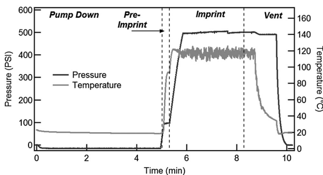
Fig. 2 Pressure and temperature cycles for the NIL process for the DNA biopolymer using the Nanonex NX-2600. The four imprint stages are: (1) pump-down where the chamber is placed under vacuum, (2) preimprint where the temperature raised to the glass transition temperature, T_g , of the material and the pressure is gradually increased, (3) imprint where the imprint pressure and temperature are applied for a set time, and (4) cool down/chamber vent where the imprint pressure is maintained until the sample is cooled.
