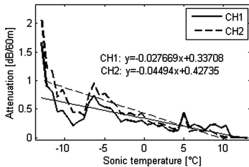
Fig. 3 Scatter plot between FSO link attenuation and sonic temperature measured on the observatory tower (receiver); three-year measurement at the Milesovka site. The CH1 curve corresponds with the 1550 nm, CH2 to 830-nm wavelength.
