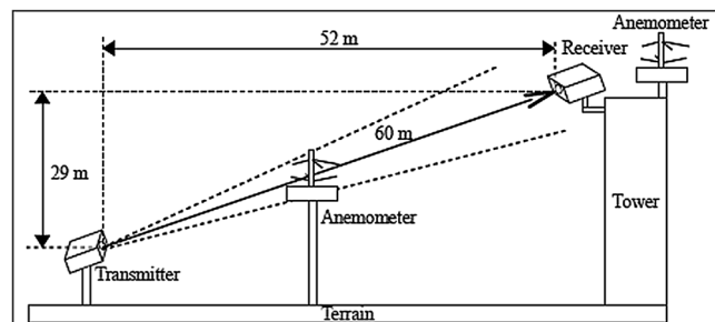
Fig. 1 Sketch of FSO link of the IAP Prague at Milesovka hill.
