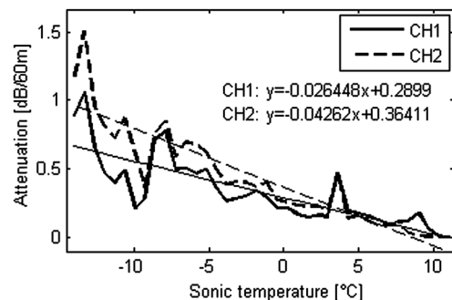
Fig. 2 Scatter plot between FSO link attenuation and sonic temperature measured on the lamp post; three-year measurement at the Milesovka observatory. The CH1 curve corresponds with the 1550 nm, CH2 to 830-nm wavelength.
