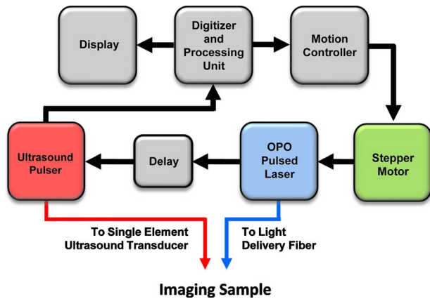
Fig. 3 Experimental setup for imaging of metal needles positioned at different angles in water and gelatin phantom. Imaging was performed with a single element US transducer (7 MHz, f/4 ). The center frequency of this transducer was similar to the imaging array used in Fig. 1. The imaging sample was irradiated with 800-nm-wavelength light. Laser fluence was also approximately 10 \text{ mJ}/\text{cm}^2 .
