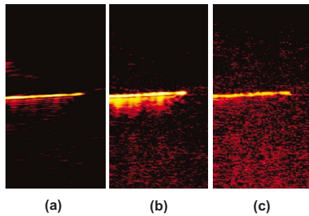
Fig. 8 PA image from Fig. 4(d) showing filtering technique to remove comet-tail artifacts; (a) unfiltered PA image of the horizontal needle. The FFT of the signal shows one frequency peak at the center frequency of the transducer (7 MHz) and one at a lower frequency around 3 MHz, representing the signal from the comet tail; (b) result of bandpass filtering demonstrating incorrect choice of cut-off frequencies (3 to 10 MHz), low-frequency components are still present, blurring out the artifacts; and (c) correct bandpass filtering (4 to 10 MHz), which eliminated the comet-tail artifact. Contrast-to-noise ratios in (a), (b), and (c) were calculated to be 39.3, 38.2, and 32.5 dB, respectively.
