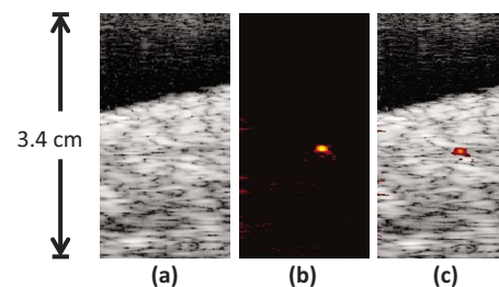
Fig. 5 Images of the hypodermic needle inserted angled approximately 15 deg with respect to horizontal. The needle is repositioned in the same tissue as in Fig. 4. The transducer is oriented at the top of the images. (a) US image of the tissue containing the needle cross section; the angled needle is not visible; (b) PA image of same cross section as (a), the highly absorbing needle appears very clearly; (c) combined US and PA image showing the exact location of the needle within the tissue. US images are displayed at 40 dB, PA images at 20 dB. Since US and PA images are obtained at the same position, the two images are spatially coregistered.
