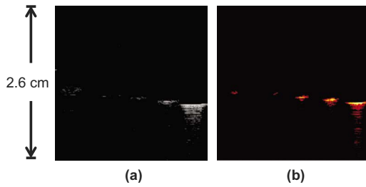
Fig. 6 Cross-sectional image of five 21 G needles in water. The needles are angled downward with respect to the horizontal plane. From left to right, needles are angled at 30, 20, 10, 5, and 0 deg, respectively.
