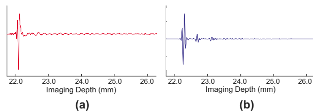
Fig. 9 Individual A-lines of the rf signal through the needle, demonstrating the nature of the comet-tail artifact. Though the images appear similar, the underlying signals are not. (a) PA A-line, the comet-tail artifact appears to be a continuous signal that diminishes over time, and (b) US A-line at the same location. The comet-tail artifact in the US image appears as a discontinuous train of signal bursts that decrease in amplitude over time.
