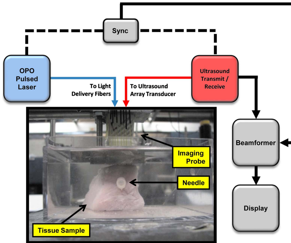
Fig. 1 Experimental setup for imaging metal needles in a porcine tissue sample. An imaging probe consisting of a 7-MHz linear array transducer and an 18-fiber bundle was positioned on the top of the sample. The pork sample was placed in a water tank for the purposes of acoustic coupling. The sample was irradiated at a 1064-nm wavelength. Laser fluence was approximately 10 \text{ mJ/cm}^2 .
