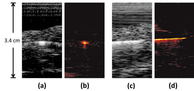
Fig. 4 Images of a hypodermic needle inserted perpendicular to the US transducer. The needle is inserted horizontally through the pork loin sample. The transducer is located toward the top of the images. (a) US image of the needle cross section in pork sample; (b) PA image of needle cross section, where the needle is easily visible; (c) US image of the needle and tissue in the transducer imaging plane; and (d) PA image of the needle in the transducer imaging plane, where the metal needle is clearly visible. The dimensions of the pork loin are approximately 30 \times 30 \times 30 \text{ mm}^3 . US images are displayed at 40 dB, PA images at 20 dB.
