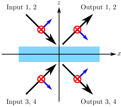
Fig. 2 Cross-sectional view of a metasurface interacting with TE- and TM-polarized plane waves.
