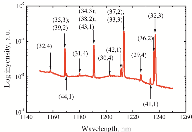
Figure 6. Low-temperature luminescence spectrum of the microring. Estimated mode orders TE_{m,n} are indicated near the peaks.
