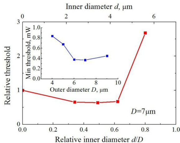
Figure 9. Room-temperature threshold (normalized to the threshold of the microdisk structure) as a function of inner diameter. Insert: the lowest threshold against the outer diameter.
