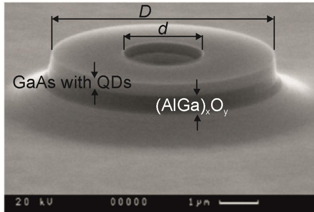
Figure 5. SEM image of QD microring laser ( D = 6\ \mu\text{m} , d = 2\ \mu\text{m} ).
