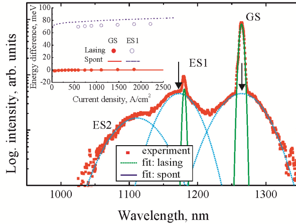
Figure 4. Emission spectrum: squares – experiment, solid curves – lasing emission, dotted curves – spontaneous emission. Insert: peak position vs current density: solid circles – GS lasing, open circles – ES1 lasing, solid curve – GS spontaneous emission, dotted curve – ES1 spontaneous emission.
