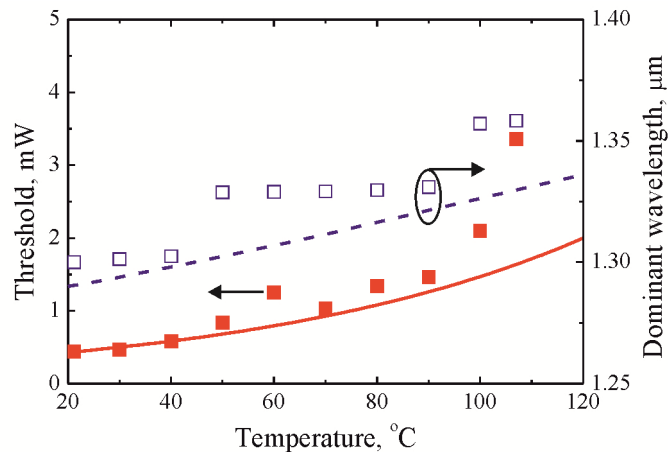
Figure 10. Temperature dependences of the threshold power (solid symbols) and wavelengths of the dominant mode (open symbols). QD ground-state optical transition against temperature (dashed curve) is also shown. Solid curve is exponential fit with T_0=65 K.
