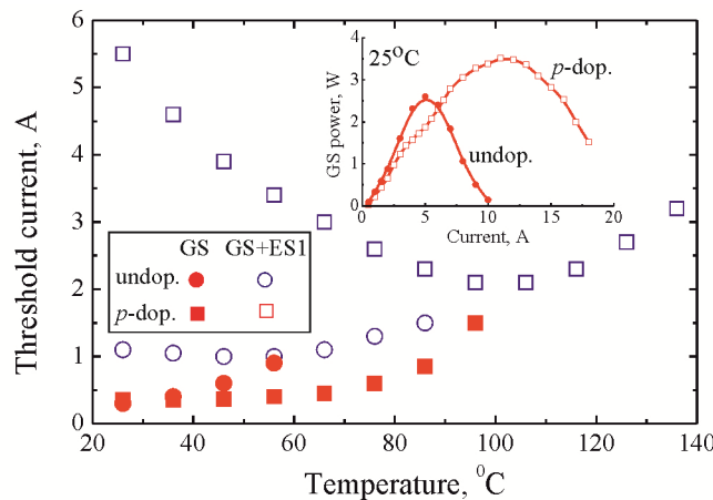
Figure 3. Threshold vs temperature for ground-state lasing (solid symbols) and two-state lasing (open symbols) in lasers with undoped (circles) and p -type doped (squares) QDs. Insert: power of the GS-line vs current.
