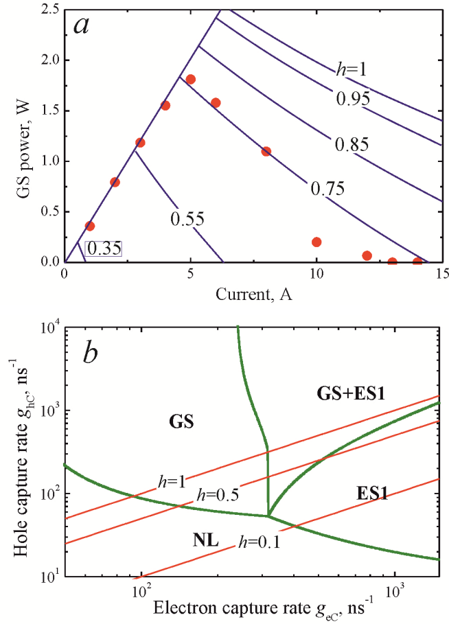
Figure 2. L - I curves for ground-state component (a): circles – experiment; lines – calculation for different ratio of hole-to-electron relaxation rates ( h ). Operation diagram of QD laser: heavy lines separates regions of different lasing regimes (NL – no lasing, GS – pure ground-state lasing, GS+ES1 – two-state lasing, ES1 – pure excited-state lasing); thin lines correspond to different h values.
