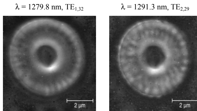
Figure 7. NSOM images demonstrating WGM modes of different orders in the microring resonator.
