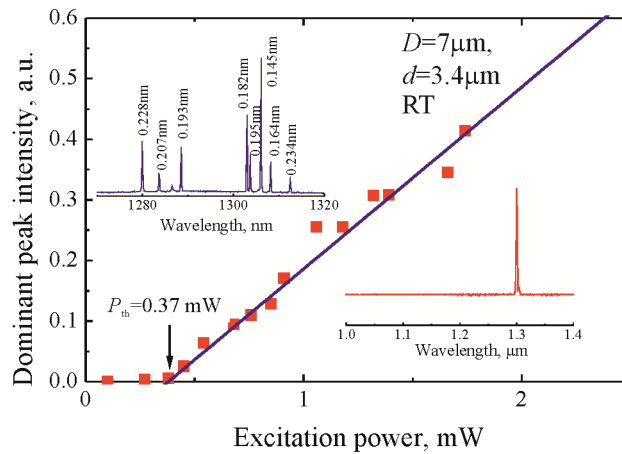
Figure 8. Intensity of the dominant mode against excitation power (symbols). Curve is a guide to the eye. Insert: luminescence spectrum below threshold (left) and above threshold (right).
