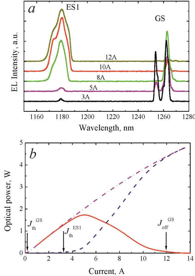
Figure 1. Lasing spectra at different currents (a); laser power (b): dashed-dotted curve – total (GS+ES1), solid curve – ground-state component (GS), dashed curve – first excited-state component (ES1).
