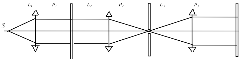
FIG.4 4F-system of pseudocolorimeter
