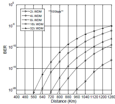
Fig. 7: Bit Error Rate
