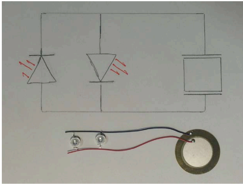
Fig. 4. Electrical diagram and components used by older participants.
