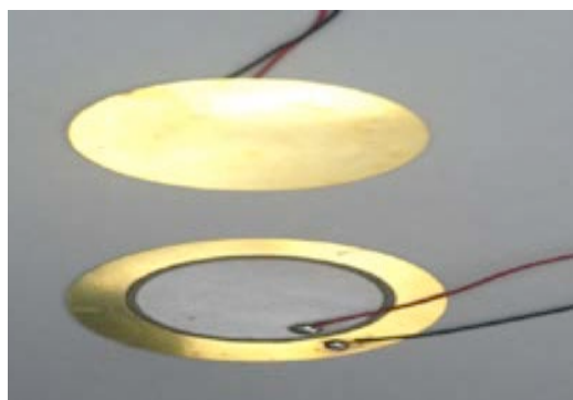
Fig. 2. Image of piezoelectric musical instrument pickups as received. Note the lightly-colored piezoelectric ceramic on one side and wire leads. The plain brass metal surface is used as the touch pad.
