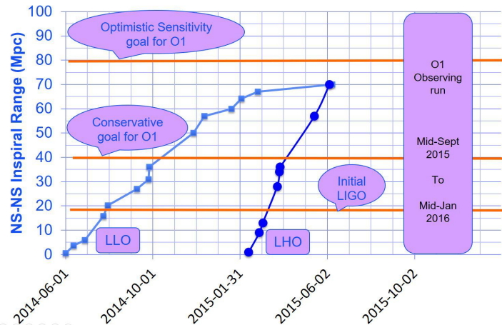
Figure 2. Commissioning progress. This graph shows the increase in binary neutron star reach as function of commissioning time, starting immediately after installation finished. The initial LIGO reach was surpassed within 2 months. The Hanford detector (LHO) finished installation about 8 months after the Livingston one (LLO), but caught up fast. Both detectors reached a sky-averaged range around 70 Mpc for binary neutron star inspirals with a single detector SNR of 8.
