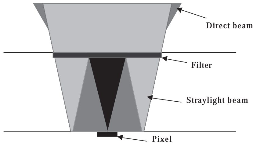
Fig. 2: infraband straylight.
