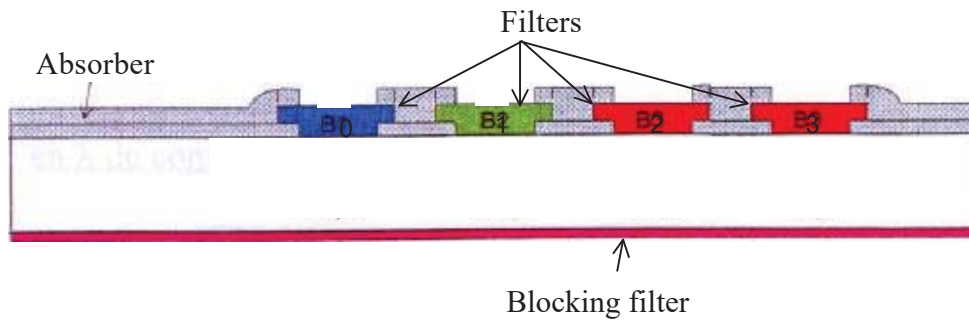
Fig. 5: overall design.
