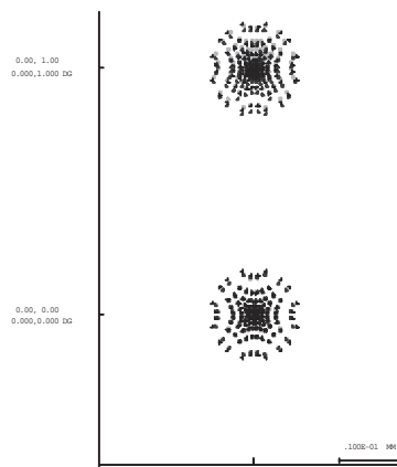
Polychromatic spot diagram after irradiation
