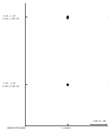
Polychromatic spot diagram before irradiation
