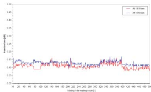
fig. 14 Reproducibility of the Mini-AVIM
