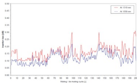
fig. 13 Reproducibility of the AVIM
