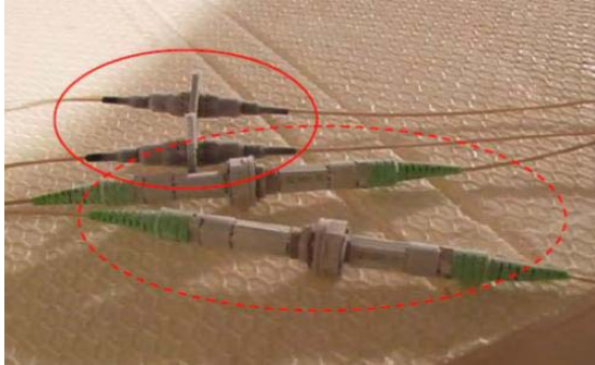
fig. 6 Mini-AVIM and AVIM during cold temperature strep stress
