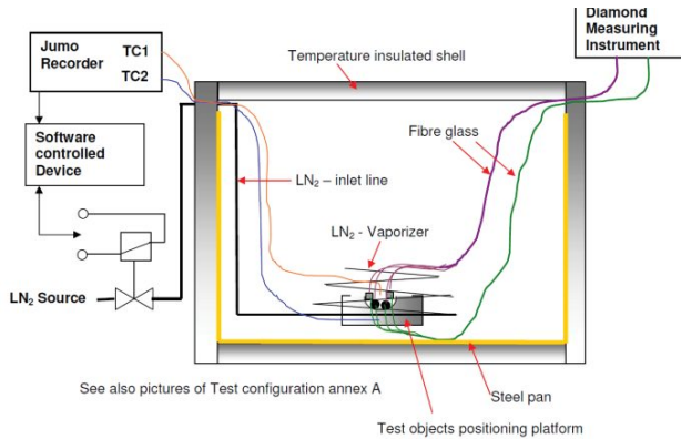
fig. 7 Cold temperature step stress setup
