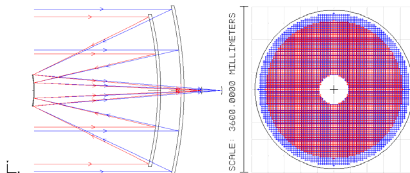
Fig. 3. Ray trace on-axis (left) and on-axis beam footprint on M1 (right) for Case 1 (blue) and 3 (red).
