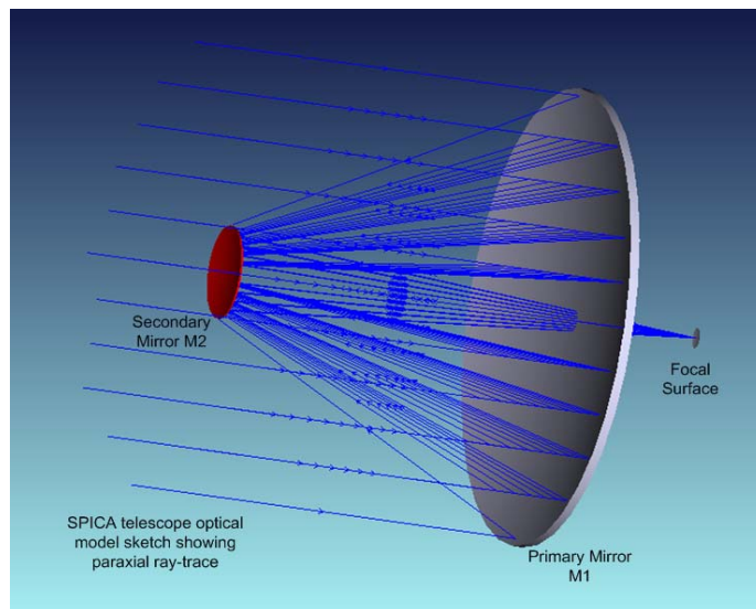
Fig. 1. STA optical design configuration and ray trace sketch. For clarity only on-axis rays are shown.
