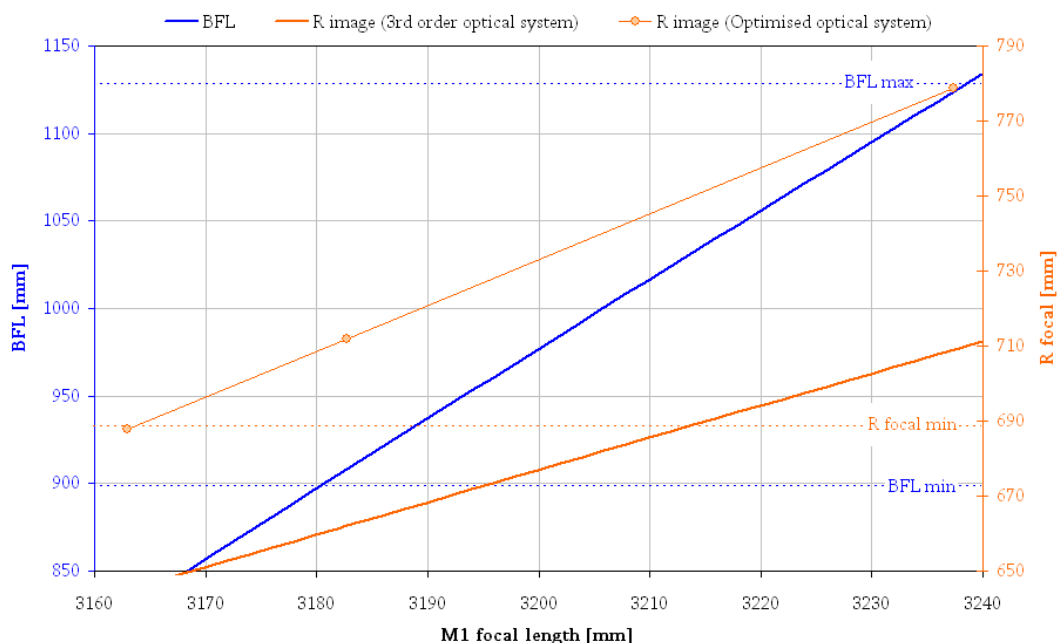
Fig. 2. BFL and R_{focal} vs. the focal length of the primary mirror.
