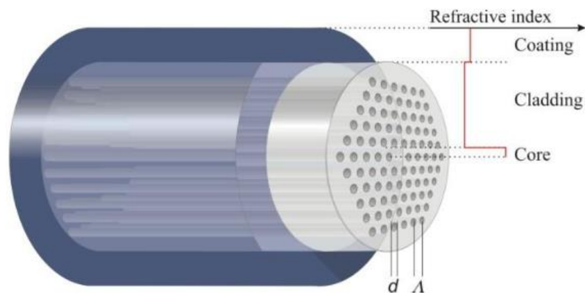
Figure 3. Schematic of the classical triangular cladding single-core photonic crystal fiber in which light is guided in a solid core embedded in a triangular lattice of air holes. The fiber structure is determined by the hole-size, d , and the hole-pitch, \Lambda . Like standard fibers, the PCF is coated with a high index polymer for protection and to strip off cladding-modes.
