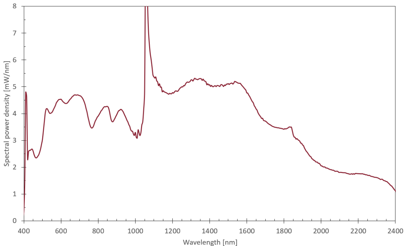
Figure 2. Spectral power density of a commercial supercontinuum laser (SuperK FIANIUM FIU-15, NKT Photonics), covering wavelengths from 400 nm to 2400 nm with around 6W integrated power. The 1064 nm spike is the residual pump peak of the Yb fiber laser.
