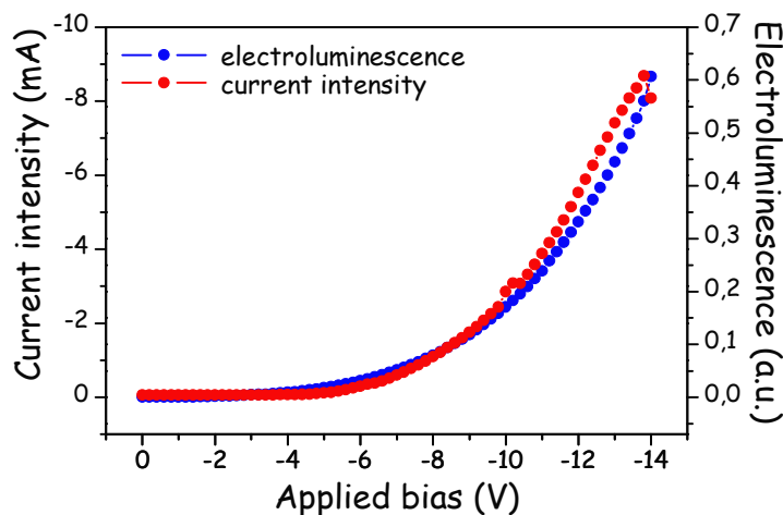
Figure 6. Opto-electronic characteristics of the OLED sketched in Figure 5a.
