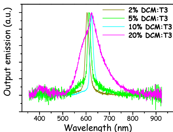
Figure 4. Normalized DCM:T3 blends emission spectra collected from the edge of a 4 mm 2 -wide excitation stripe. The pump intensity is higher than the ASE threshold.
