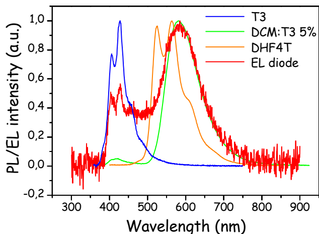
Figure 7 Electroluminescence spectrum of the OLED compared with the photoluminescence spectra of the single layers composing the overall heterostructure.
