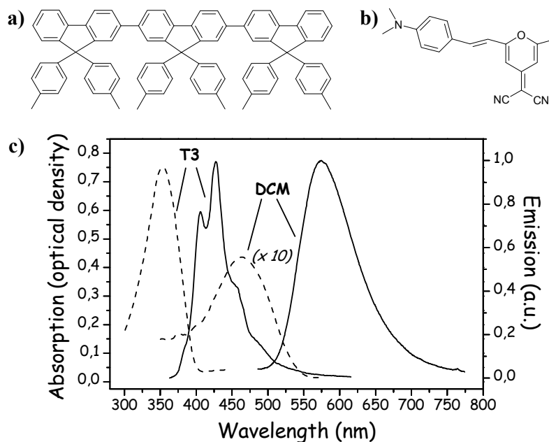
Figure 1. Chemical structure of (a) ter(9,9-diarylfuorene) (T3) and (b) 4-(dicyanomethylene)-2-methyl-6-(p-dimethylaminostyryl)-4H-pyran (DCM). c) Absorption spectra (dashed line) and photoluminescence spectra (solid line) of a 10^{-3} M solution of DCM molecules dissolved in dichloromethane and of a 100 nm-thick T3 film grown by thermal evaporation.
