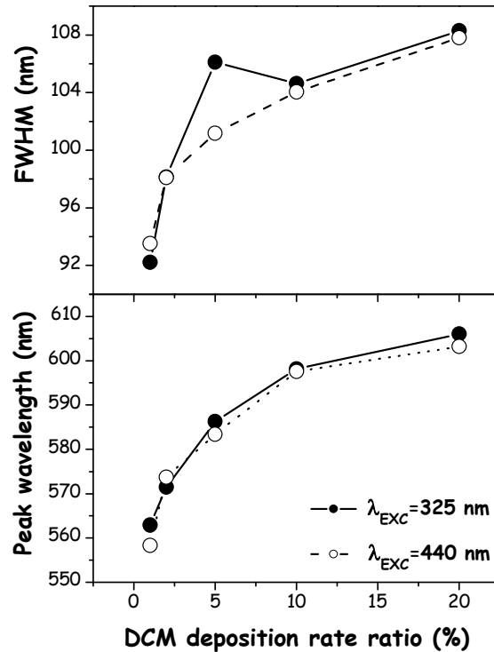
Figure 3. Full width at half maximum (FWHM) values and peak wavelengths of DCM photoluminescence maxima with increasing DCM concentration. Donor and the acceptor molecules are selectively excited at 325 nm and 440 nm.
