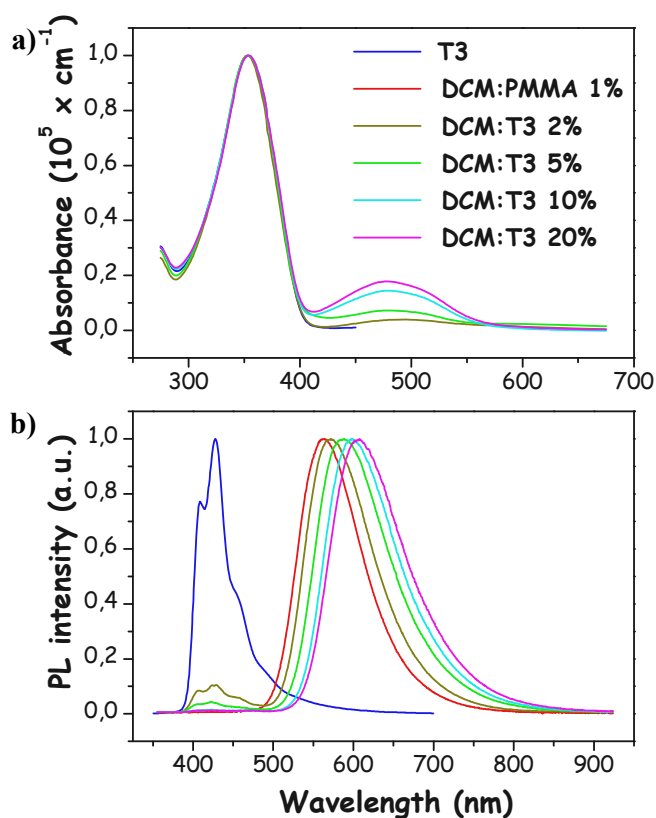
Figure 2. a) Absorption spectra of thin films of different DCM:T3 blends with increasing DCM molar concentration and of T3 alone. All the spectra are normalized with respect to T3 alone absorption peak. b) Photoluminescence spectra of thin films of different DCM:T3 blends with increasing DCM molar concentration obtained by exciting the donor component. The spectra of neat T3 thin-film and of the solid solution of DCM dispersed in PMMA at 1% in weight are reported. Photoluminescence spectra are normalized with respect their own maxima.
