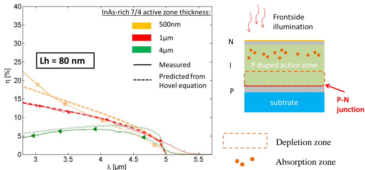
Fig 4 Left : comparison between QE measurements and predictions from Hovel equations for three InAs-rich photodiodes with different active zone thicknesses (500 nm, 1 μm and 4 μm), at 77K and 0V bias voltage; Right : schematic view of the front-side illuminated InAs-rich photodiode.
