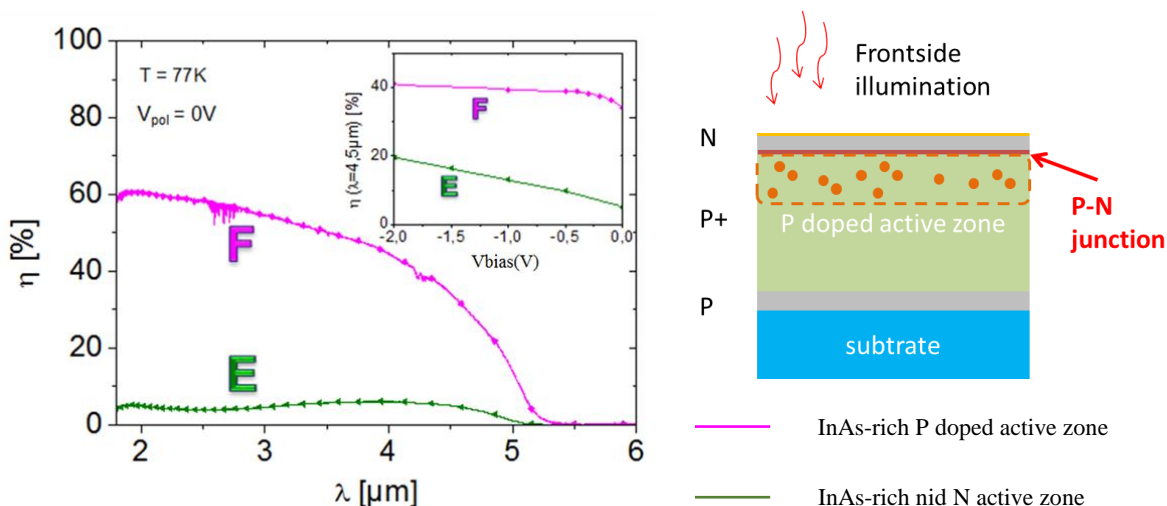
Fig 5 Left : QE measurements on InAs-rich T2SL photodiodes with non intentionally doped or P doped active zone at 77K and V bias =0V ; Right : schematic view of the front-side illuminated InAs-rich photodiode (the p-n junction is now at the i/n interface, allowing a good overlap between the absorption and the collection zones).
