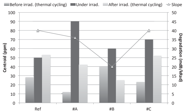
Figure 6. Centroid behavior during thermal cycling and irradiation – slope degradation
