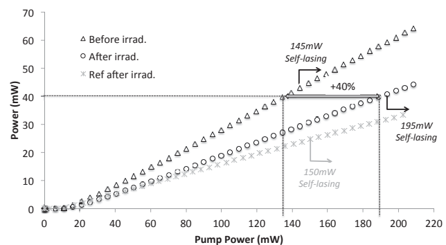
Figure 3. ASE source efficiency comparison (#B before-after irradiation, and Ref after irradiation, only)
