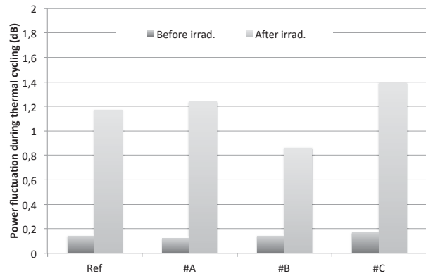
Figure 5. Output power ASE behaviour during thermal cycling (#B)
