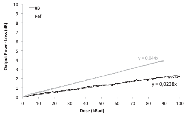
Figure 2. Dependence of the output power loss versus radiation
