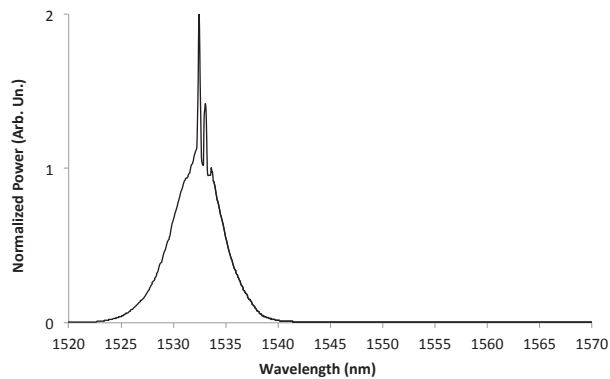
Figure 8. Self-lasing observation from over pumped source
