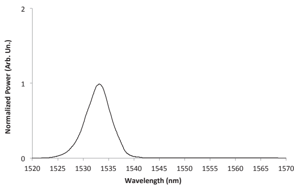
Figure 1. ASE spectrum from optimized source
