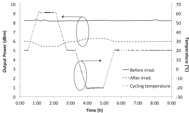
Figure 4. Output power ASE behaviour during thermal cycling (#B)
